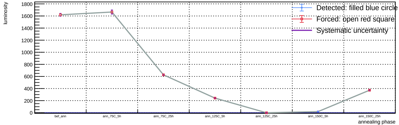
Sensor B1, v = 3 V, representative T = 23 C (max available) - Spot 115: luminosity vs phase
