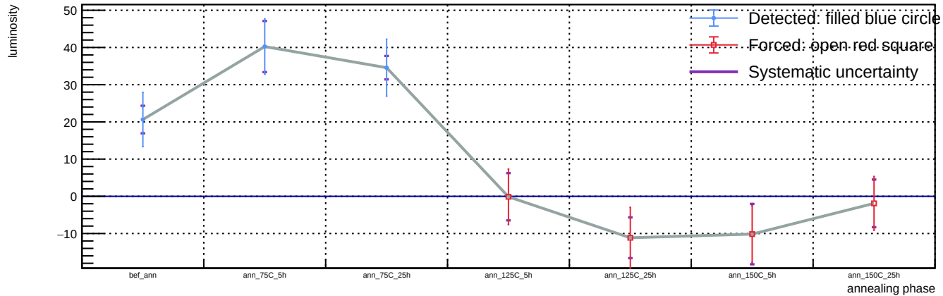
Sensor B1, v = 3 V, representative T = 23 C (max available) - Spot 19: luminosity vs phase
