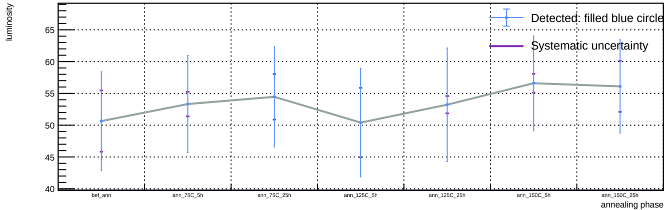
Sensor B1, v = 3 V, representative T = 23 C (max available) - Spot 21: luminosity vs phase
