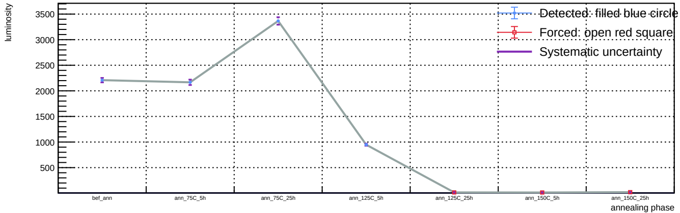
Sensor B1, v = 3 V, representative T = 23 C (max available) - Spot 25: luminosity vs phase
