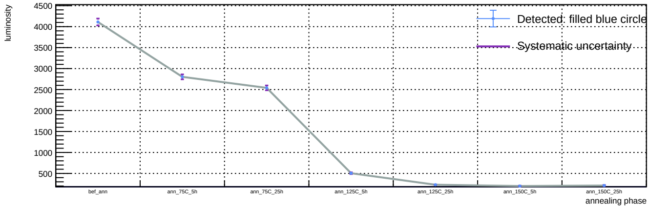
Sensor B1, v = 3 V, representative T = 23 C (max available) - Spot 30: luminosity vs phase
