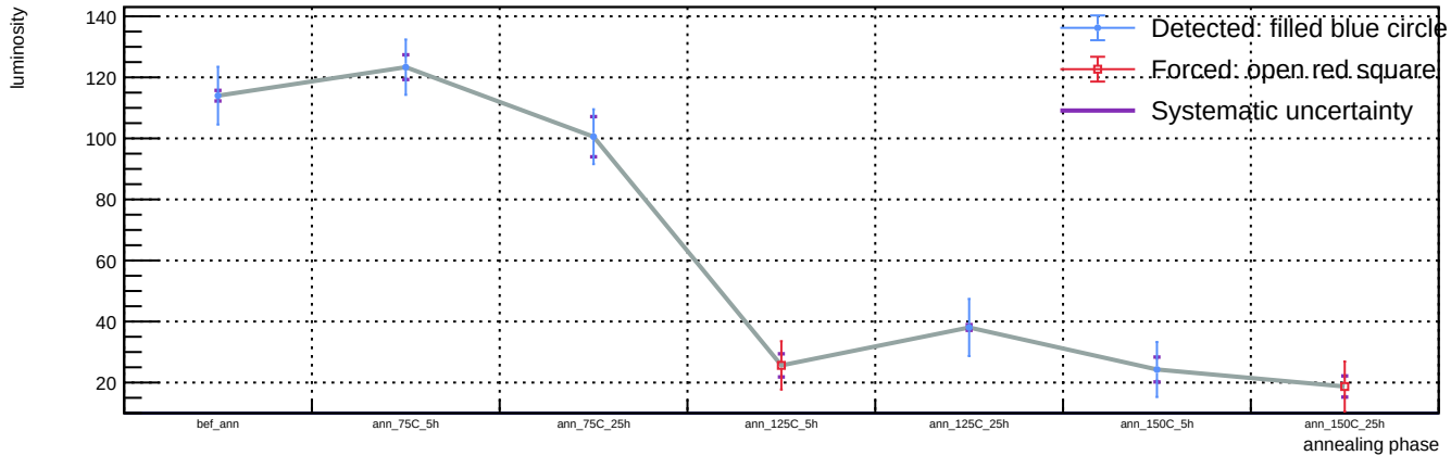
Sensor B1, v = 3 V, representative T = 23 C (max available) - Spot 33: luminosity vs phase
