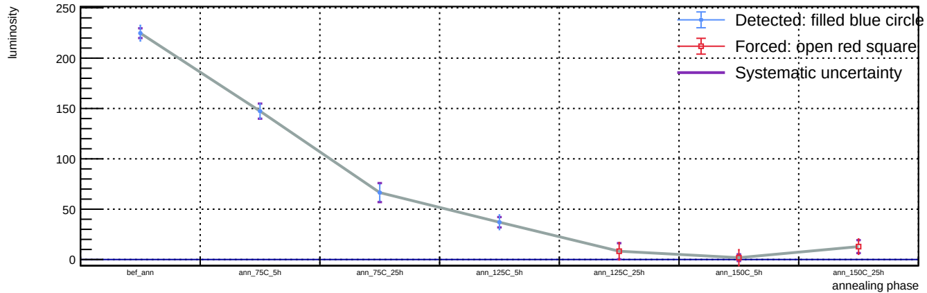
Sensor B1, v = 3 V, representative T = 23 C (max available) - Spot 37: luminosity vs phase
