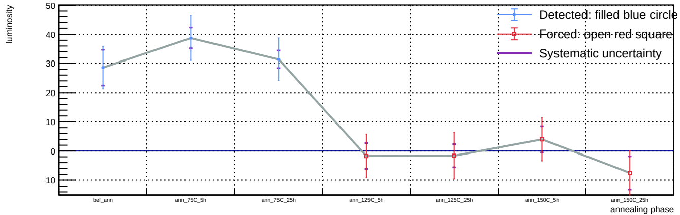
Sensor B1, v = 3 V, representative T = 23 C (max available) - Spot 41: luminosity vs phase
