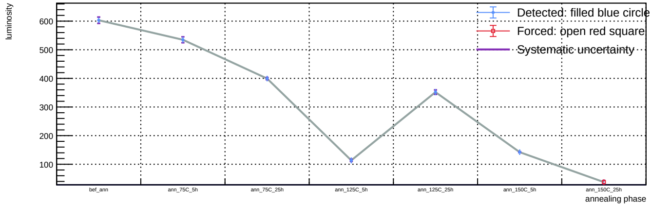
Sensor B1, v = 3 V, representative T = 23 C (max available) - Spot 45: luminosity vs phase
