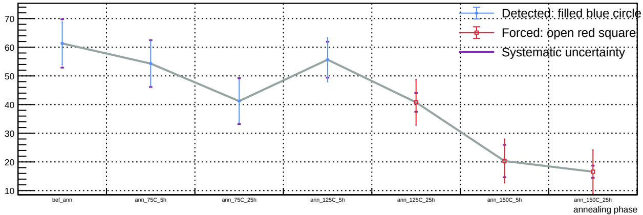
Sensor B1, v = 3 V, representative T = 23 C (max available) - Spot 46: luminosity vs phase
