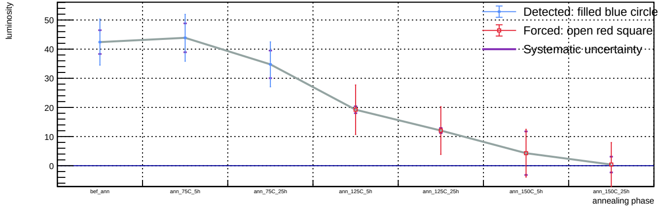
Sensor B1, v = 3 V, representative T = 23 C (max available) - Spot 50: luminosity vs phase
