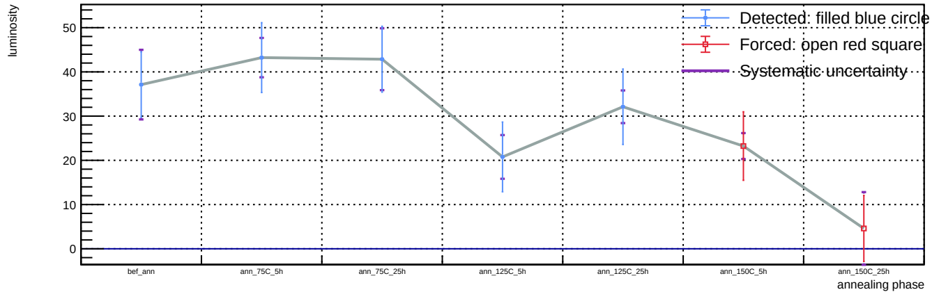
Sensor B1, v = 3 V, representative T = 23 C (max available) - Spot 51: luminosity vs phase
