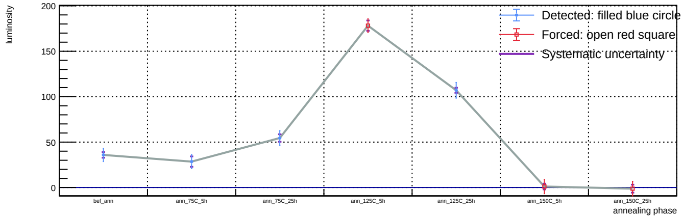
Sensor B1, v = 3 V, representative T = 23 C (max available) - Spot 52: luminosity vs phase
