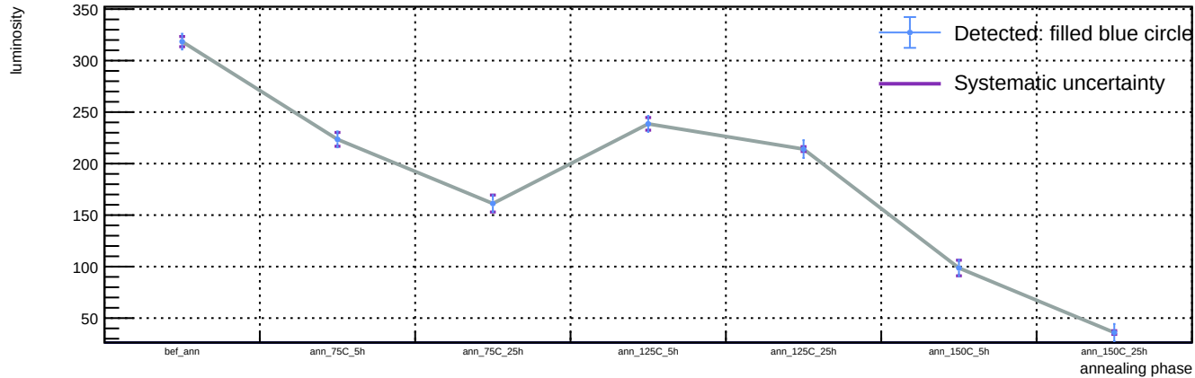
Sensor B1, v = 3 V, representative T = 23 C (max available) - Spot 53: luminosity vs phase
