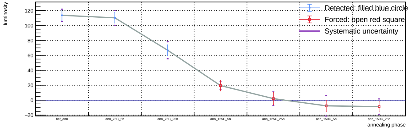
Sensor B1, v = 3 V, representative T = 23 C (max available) - Spot 55: luminosity vs phase
