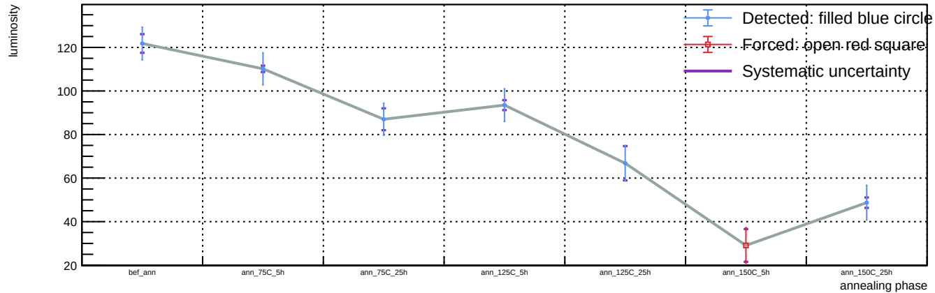
Sensor B1, v = 3 V, representative T = 23 C (max available) - Spot 6: luminosity vs phase
