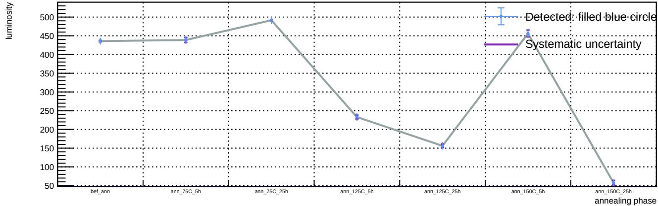
Sensor B1, v = 3 V, representative T = 23 C (max available) - Spot 60: luminosity vs phase
