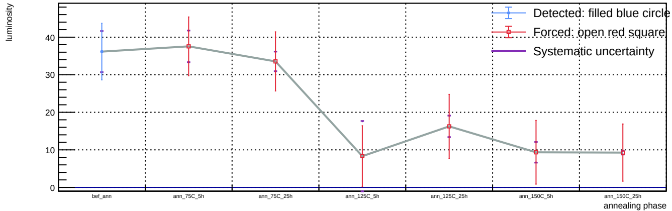
Sensor B1, v = 3 V, representative T = 23 C (max available) - Spot 62: luminosity vs phase
