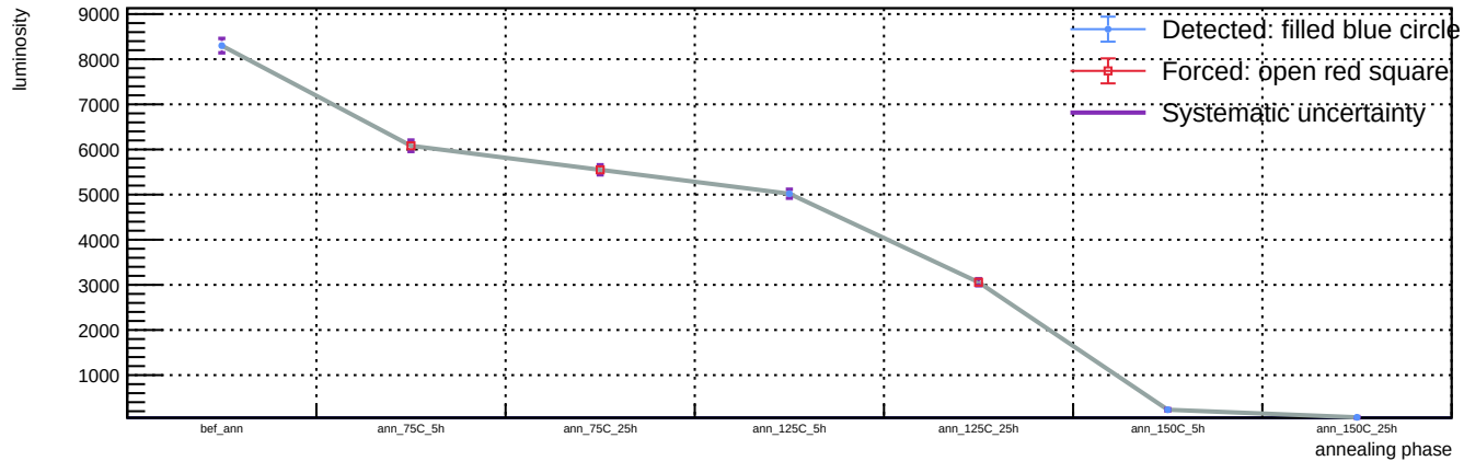
Sensor B1, v = 3 V, representative T = 23 C (max available) - Spot 63: luminosity vs phase
