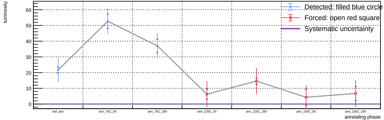
Sensor B1, v = 3 V, representative T = 23 C (max available) - Spot 66: luminosity vs phase
