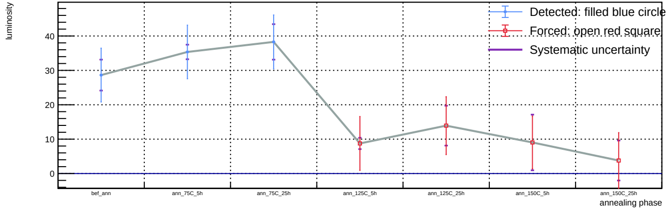
Sensor B1, v = 3 V, representative T = 23 C (max available) - Spot 67: luminosity vs phase
