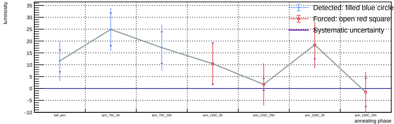
Sensor B1, v = 3 V, representative T = 23 C (max available) - Spot 69: luminosity vs phase
