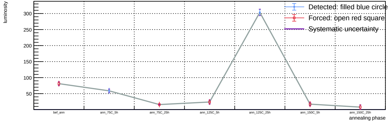
Sensor B1, v = 3 V, representative T = 23 C (max available) - Spot 70: luminosity vs phase
