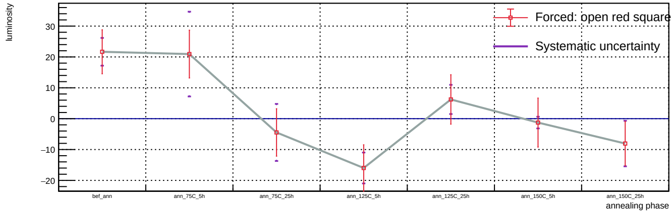
Sensor B1, v = 3 V, representative T = 23 C (max available) - Spot 72: luminosity vs phase
