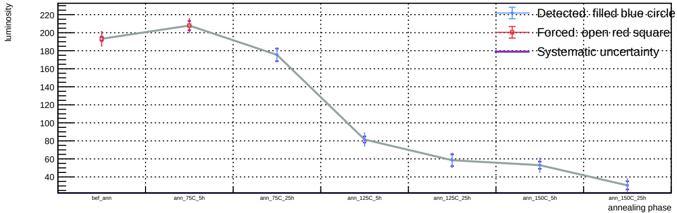
Sensor B1, v = 3 V, representative T = 23 C (max available) - Spot 74: luminosity vs phase
