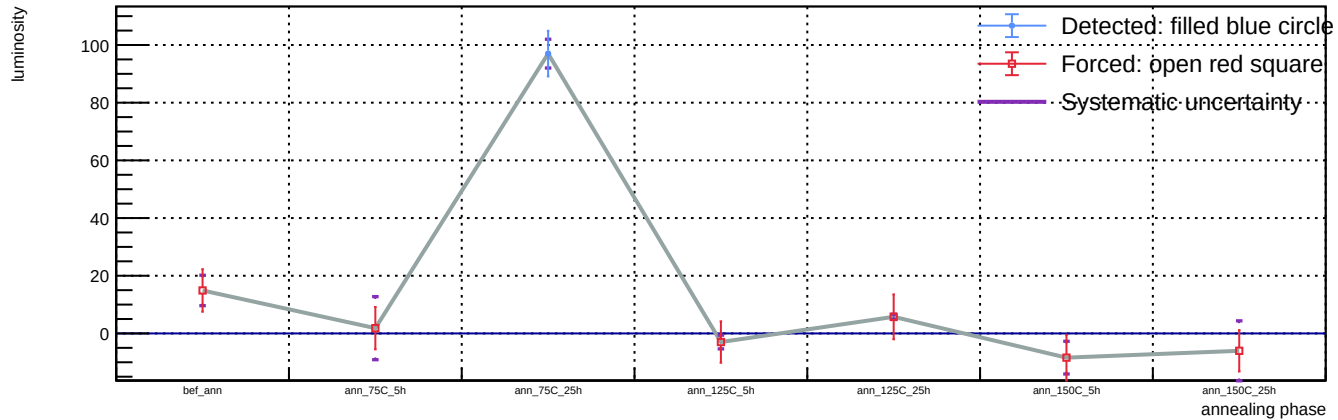
Sensor B1, v = 3 V, representative T = 23 C (max available) - Spot 76: luminosity vs phase
