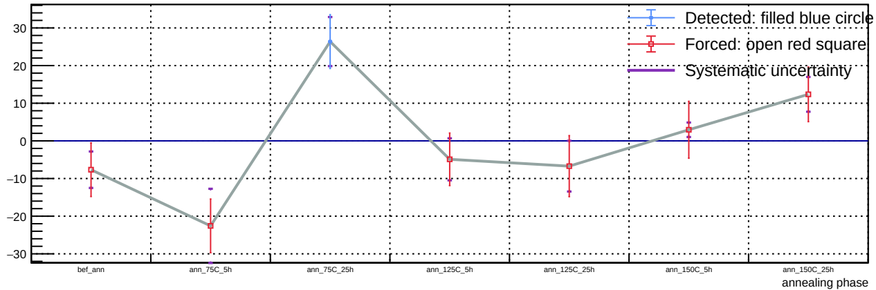
Sensor B1, v = 3 V, representative T = 23 C (max available) - Spot 77: luminosity vs phase
