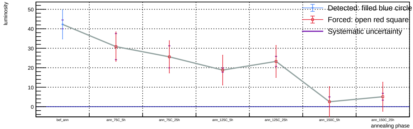
Sensor B1, v = 3 V, representative T = 23 C (max available) - Spot 8: luminosity vs phase
