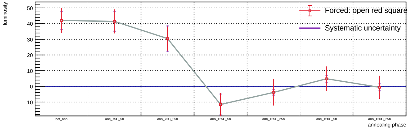
Sensor B1, v = 3 V, representative T = 23 C (max available) - Spot 81: luminosity vs phase
