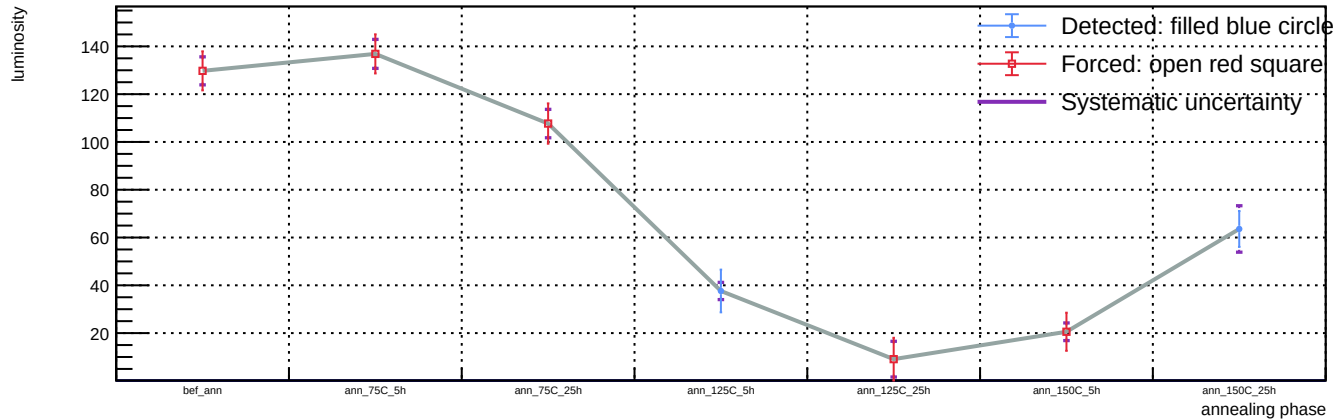
Sensor B1, v = 3 V, representative T = 23 C (max available) - Spot 88: luminosity vs phase
