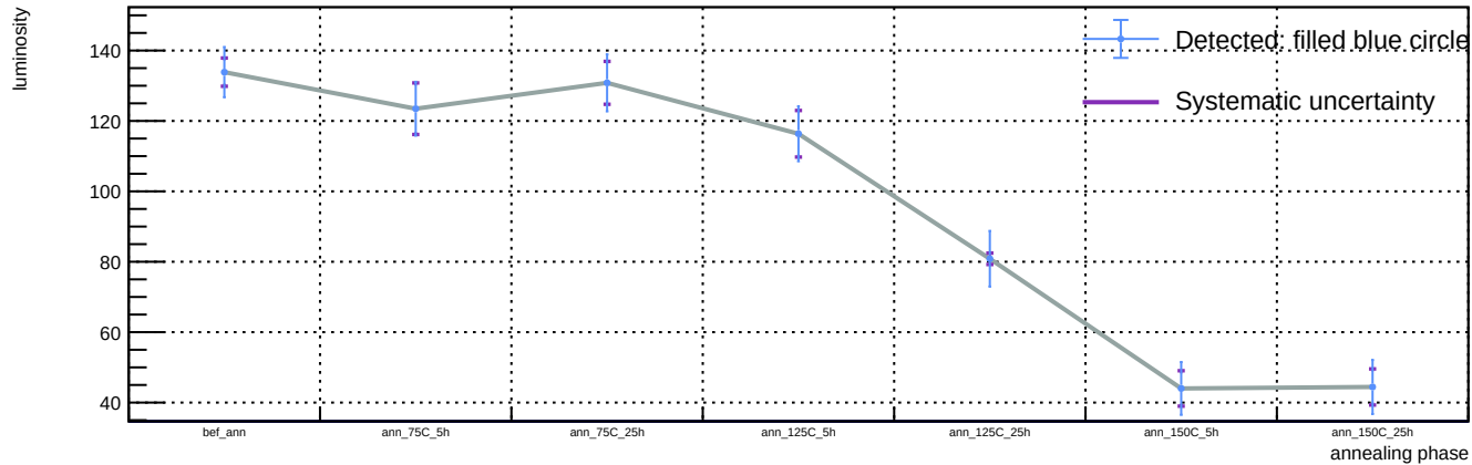
Sensor B1, v = 3 V, representative T = 23 C (max available) - Spot 9: luminosity vs phase
