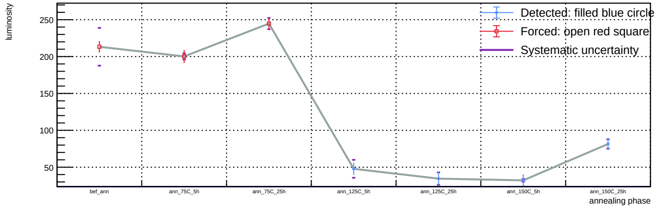
Sensor B1, v = 3 V, representative T = 23 C (max available) - Spot 94: luminosity vs phase
