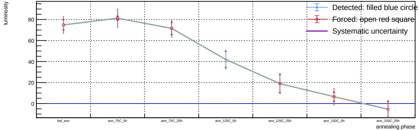
Sensor B1, v = 3 V, representative T = 23 C (max available) - Spot 95: luminosity vs phase
