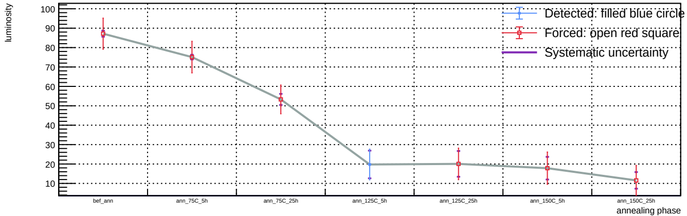
Sensor B1, v = 3 V, representative T = 23 C (max available) - Spot 99: luminosity vs phase
