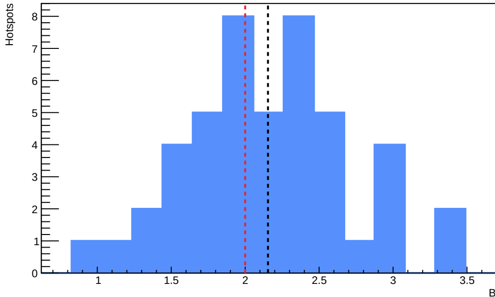
Sensor A1 - Distribution of fitted B - annealing_T=100_h=5
