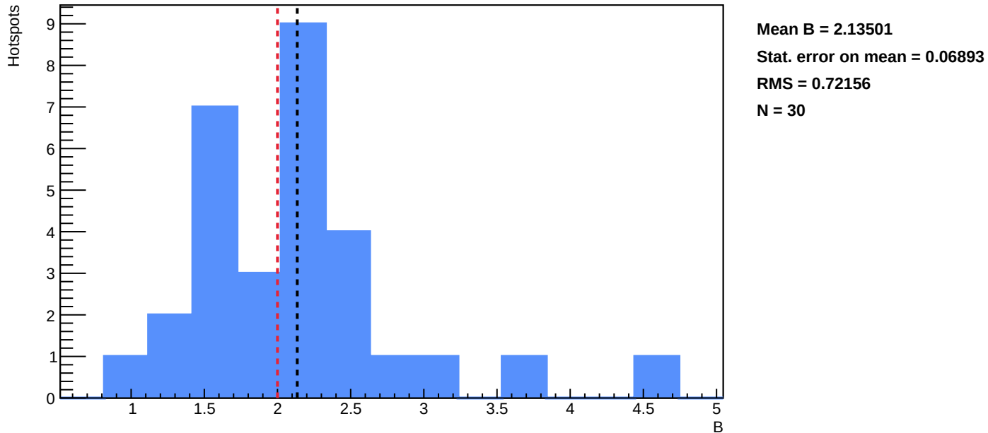
Sensor A1 - Distribution of fitted B - annealing_T=125_h=25
