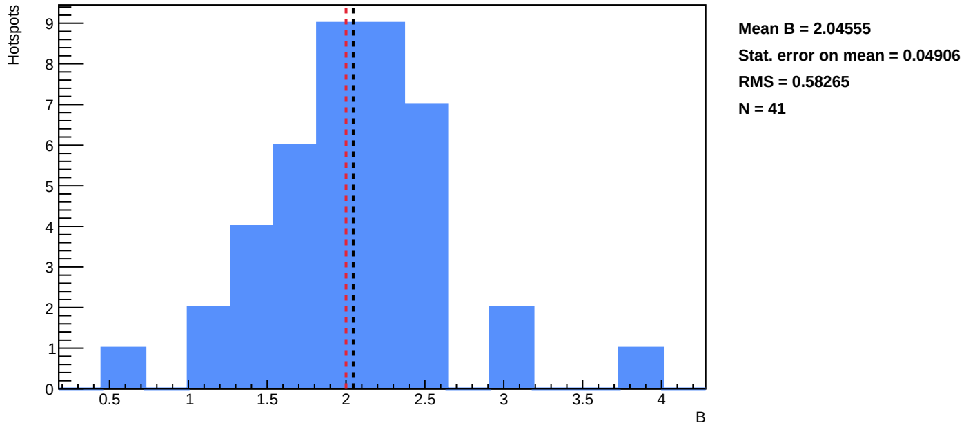
Sensor A1 - Distribution of fitted B - annealing_T=125_h=5
