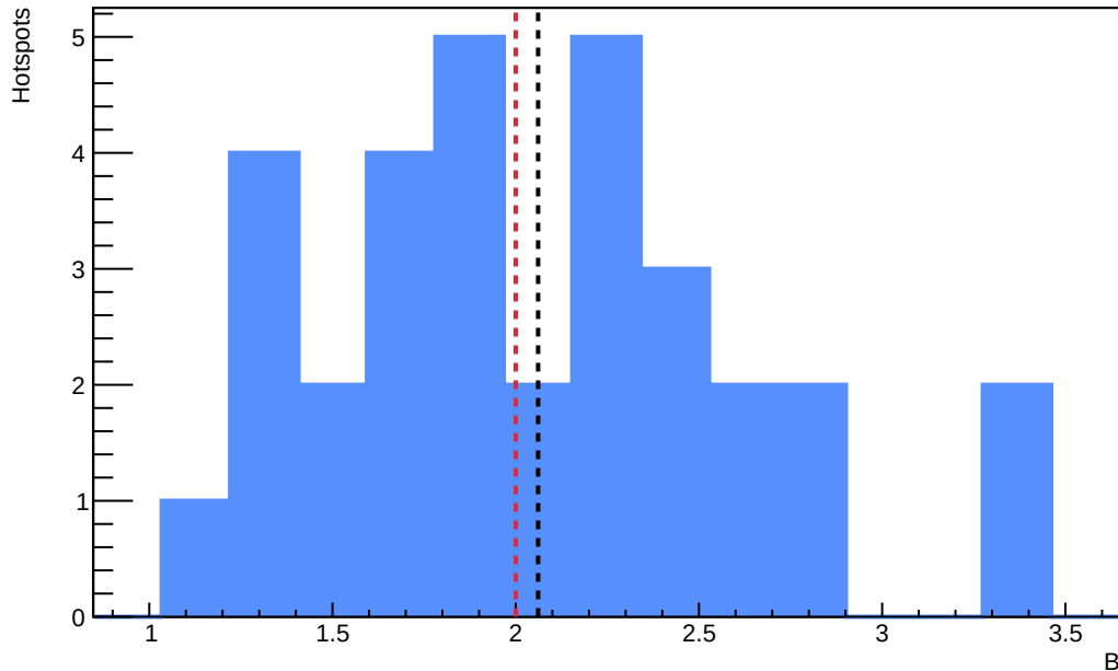
Sensor A1 - Distribution of fitted B - annealing_T=150_h=25
