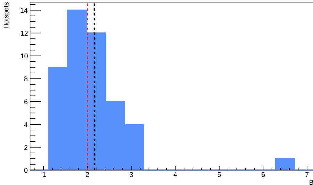
Sensor A1 - Distribution of fitted B - annealing_T=75_h=25
