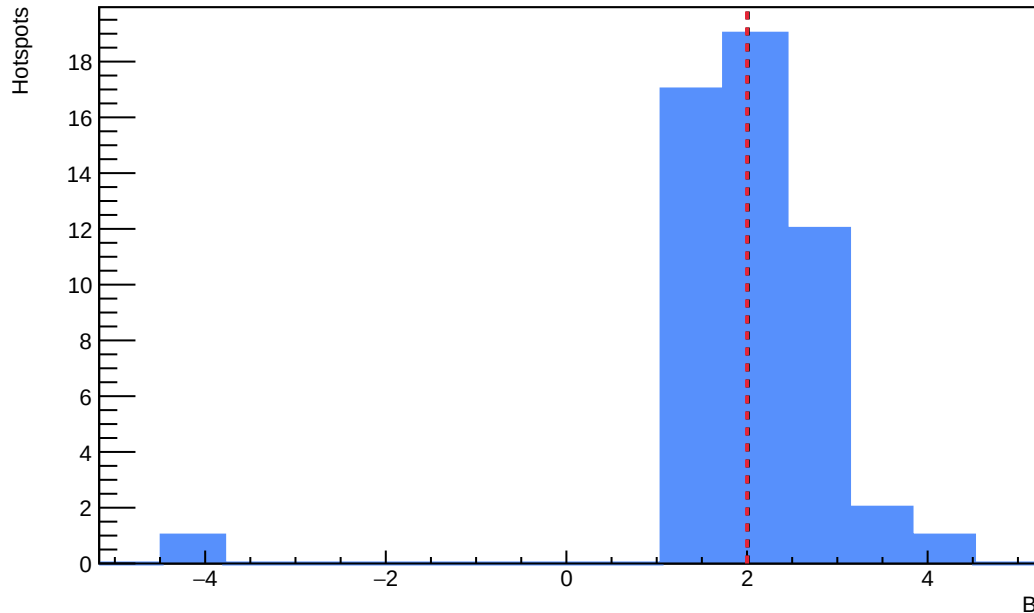
Sensor A1 - Distribution of fitted B - before_annealing
