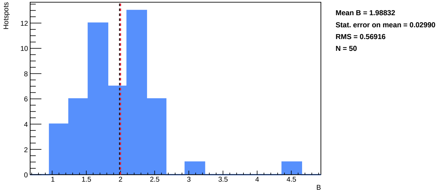
Sensor B1 - Distribution of fitted B - annealing_T=100_h=5
