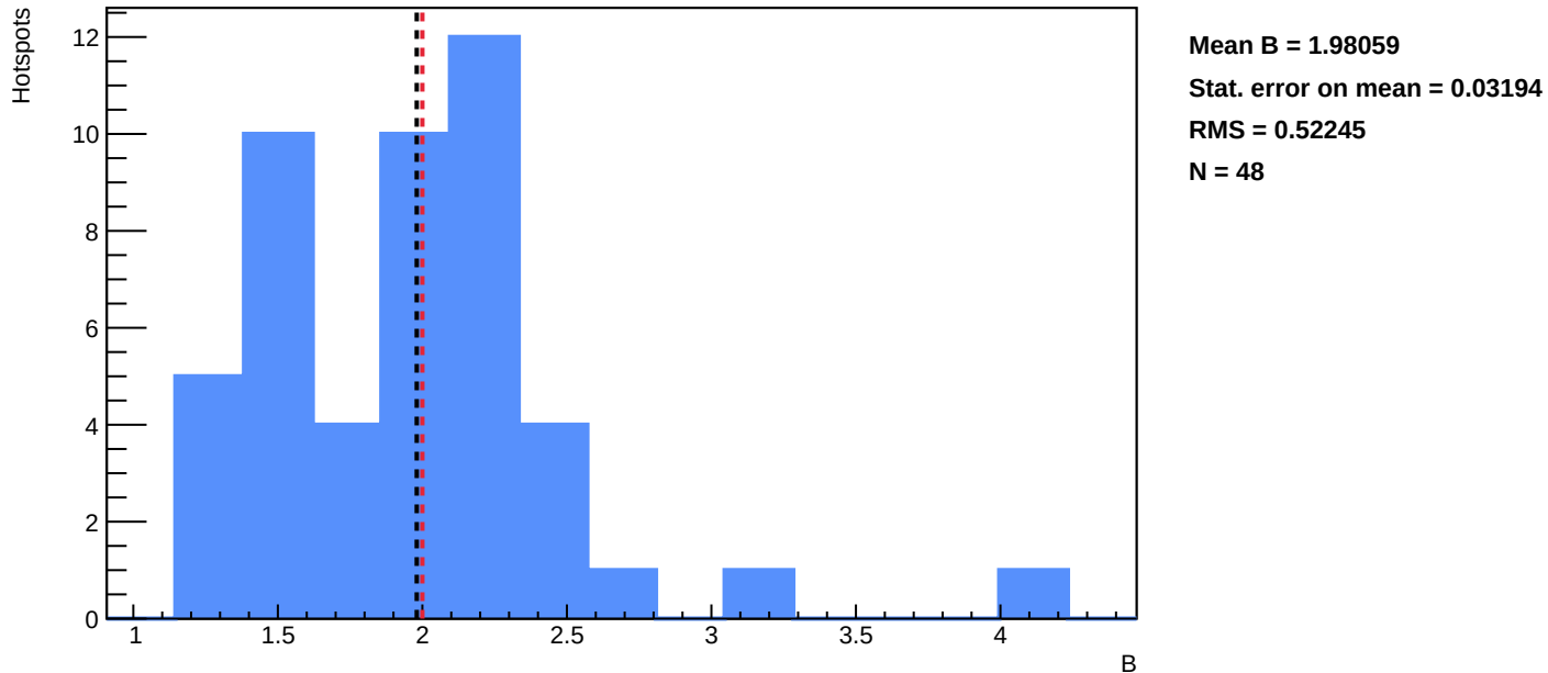
Sensor B1 - Distribution of fitted B - annealing_T=125_h=5
