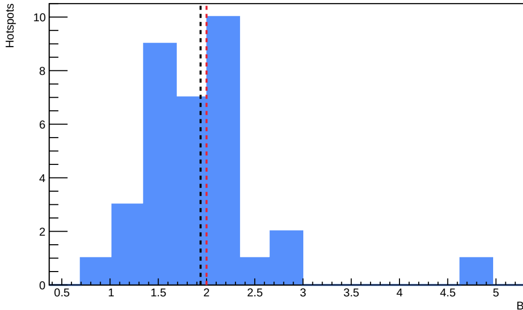
Sensor B1 - Distribution of fitted B - annealing_T=150_h=25
