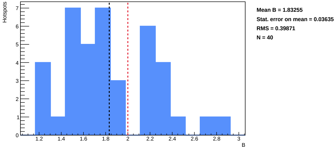
Sensor B1 - Distribution of fitted B - annealing_T=150_h=5
