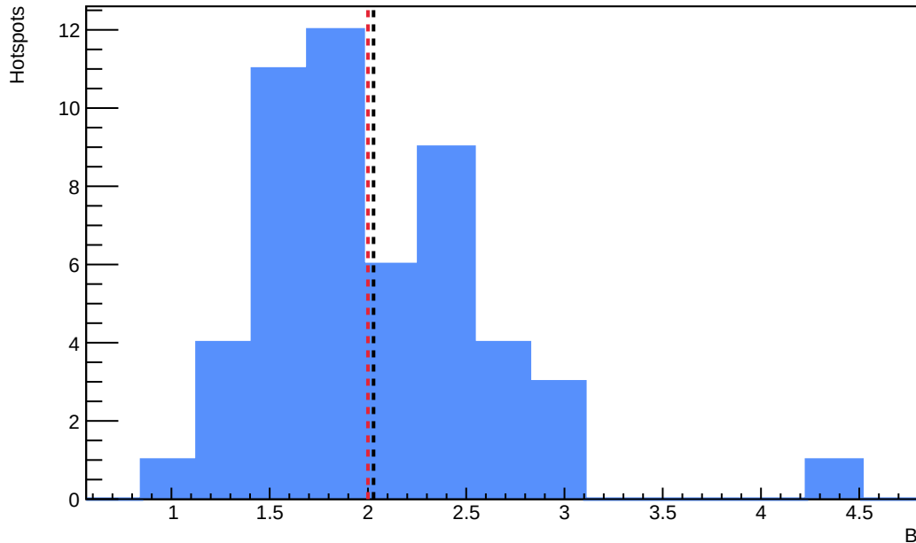
Sensor B1 - Distribution of fitted B - annealing_T=75_h=5
