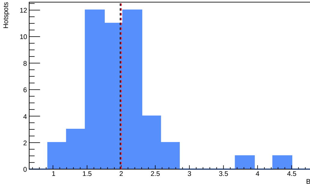
Sensor B1 - Distribution of fitted B - before_annealing
