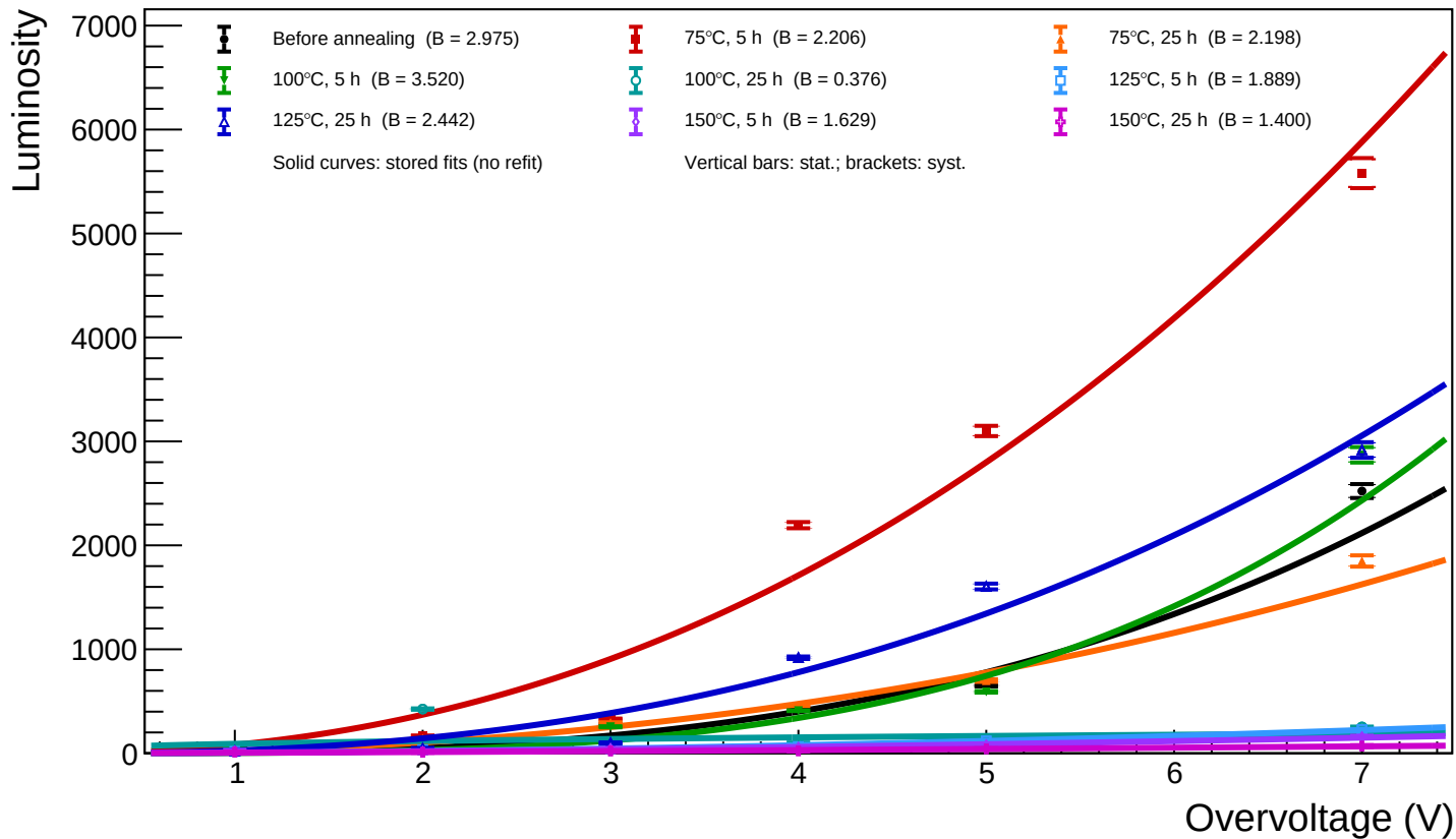
A1_T=20 - Spot 0 (x = 67.69, y = 809.36): luminosity vs overvoltage for all annealing phases
