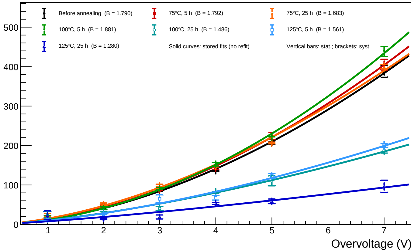
A1_T=20 - Spot 10 ( x = 415.88 , y = 948.71 ): luminosity vs overvoltage for all annealing phases
