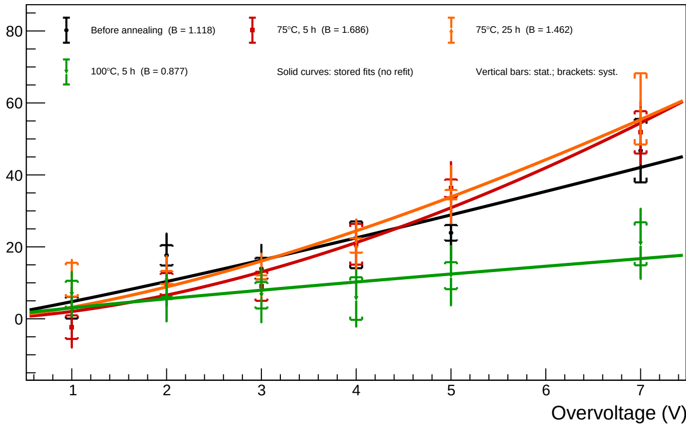
A1_T=20 - Spot 11 ( x = 417.69 , y = 550.15 ): luminosity vs overvoltage for all annealing phases
