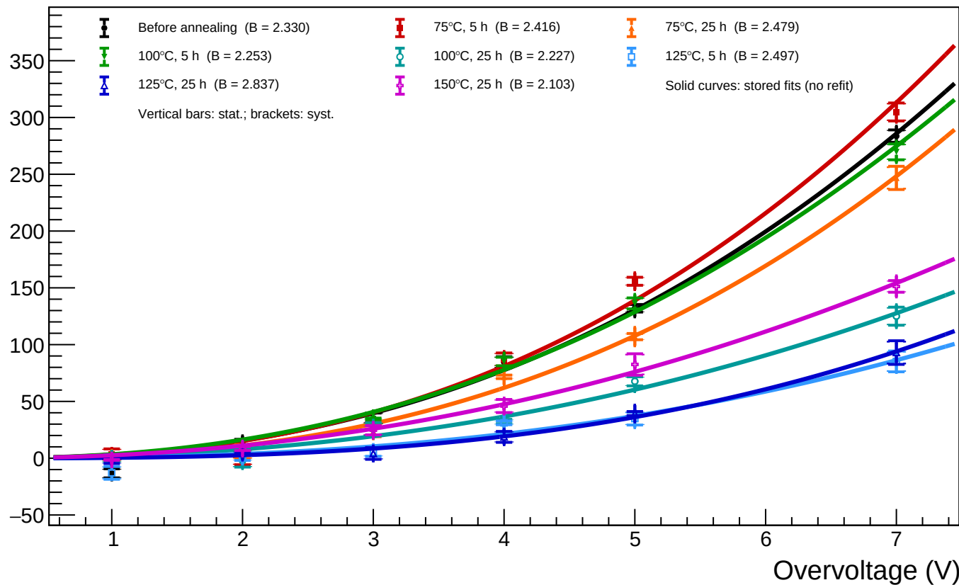
A1_T=20 - Spot 12 (x = 425.53, y = 73.12): luminosity vs overvoltage for all annealing phases
